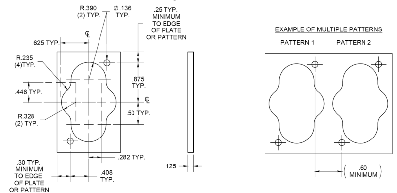
Panel Mounting Template for 4 Port Manifold (M1500-DIxxxx with optional flushing ports)
