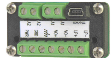
Analog Connector
