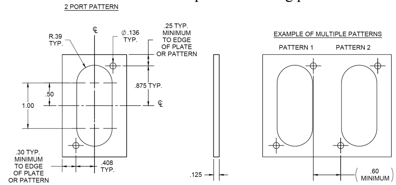
Panel Mounting Template for 2 Port Manifold
